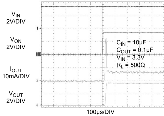
Figure 15. t_{dON} Response
