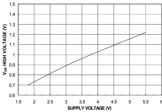
Figure 3. V_{ON} High Voltage vs. Input Voltage
