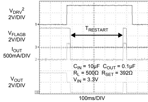
Figure 14. T_{RESTART} Response
