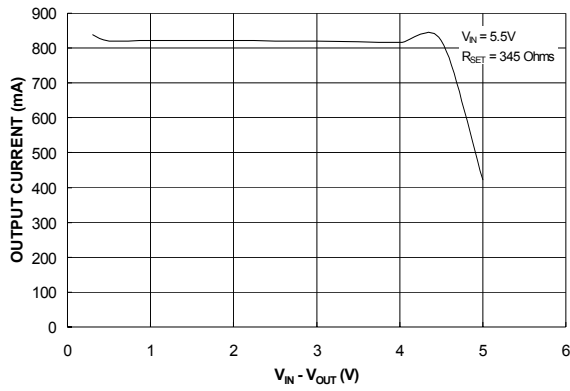
Figure 7. Current Limit vs. Output Voltage
