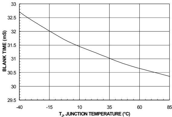
Figure 11. T_{BLANK} vs. Temperature
