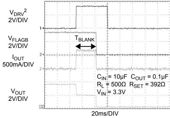
Figure 13. T_{BLANK} Response
