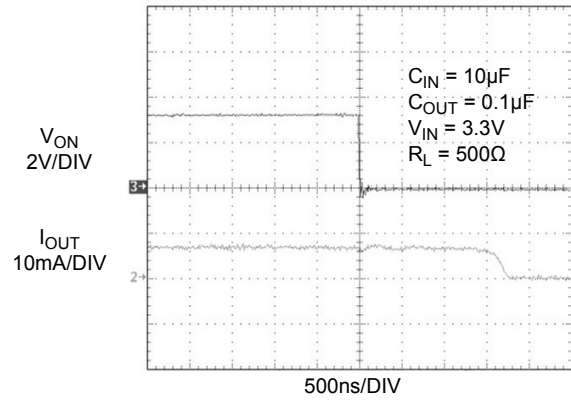
Figure 16. t_{dOFF} Response
