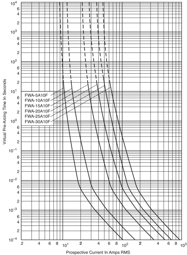
Time-Current Curve
