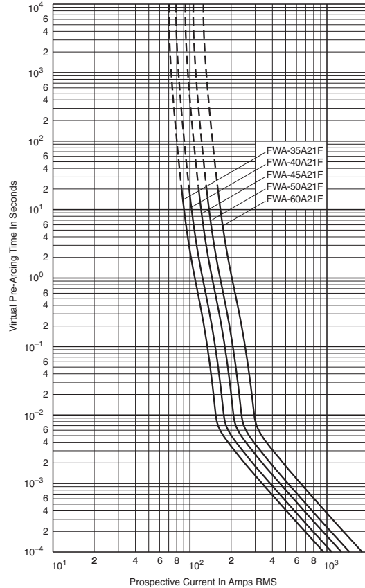
Time-Current Curve
