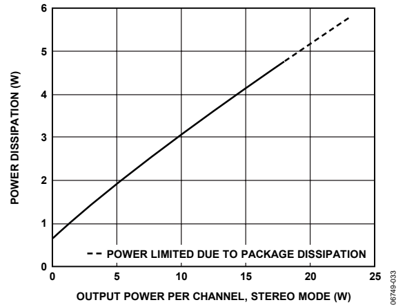
Figure 33. Power Dissipation vs. Output Power, 15 V, 6 Ω, Stereo Mode, Both Channels Driven
