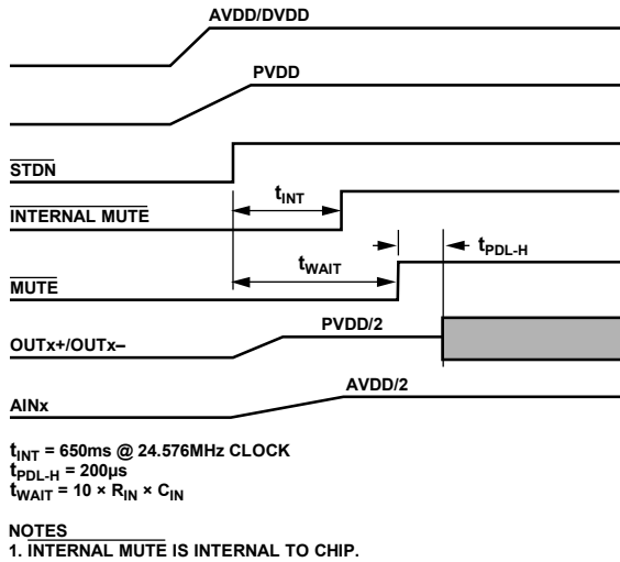
Figure 46. Recommended Power-Up Sequence
