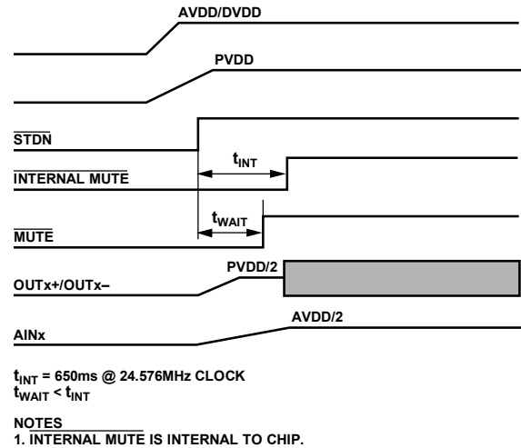
Figure 47. Power-Up Sequence, t_{WAIT} < t_{INT}
