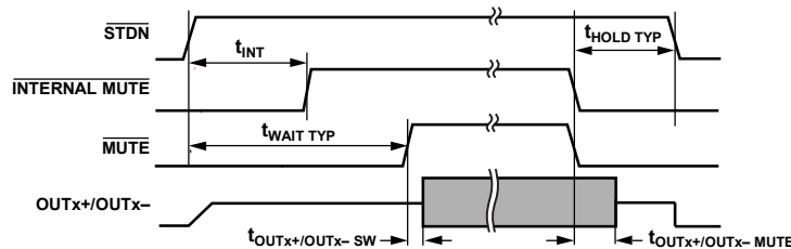
Figure 3. Timing Diagram (Typical)
