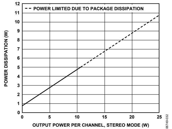
Figure 32. Power Dissipation vs. Output Power, 15 V, 4 Ω, Stereo Mode, Both Channels Driven
