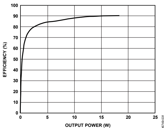
Figure 31. Efficiency vs. Output Power, 15 V, 8 Ω
