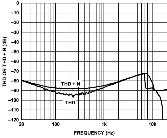
Figure 23. THD or THD + N vs. Frequency @ 1 W, 4 Ω, PVDD = 15 V, PGA = 0 dB
