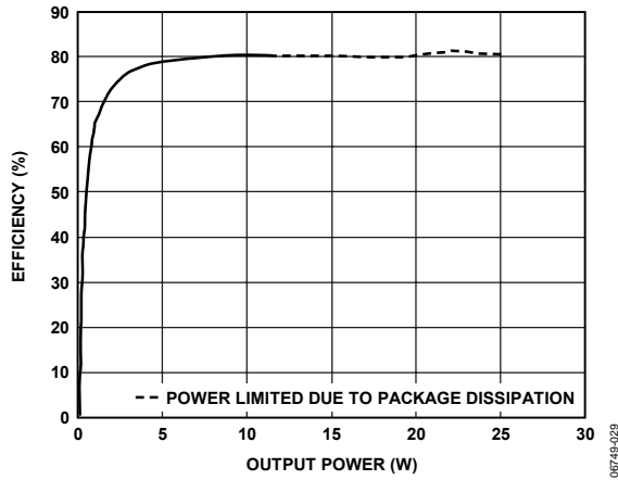
Figure 29. Efficiency vs. Output Power, 15 V, 4 Ω
