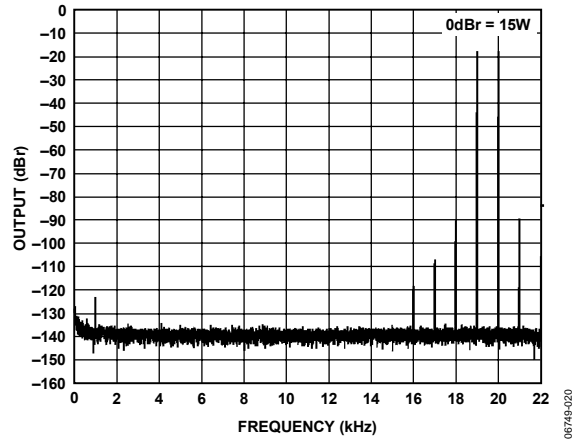
Figure 20. FFT @ 1 W, 6 Ω, PVDD = 15 V, PGA = 0 dB, 19 kHz and 20 kHz Sine
