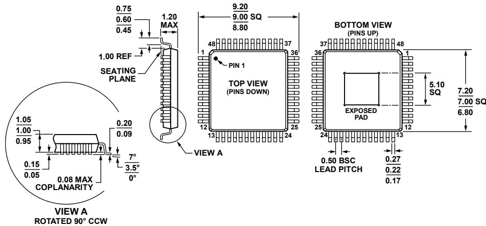
Figure 52. 48-Lead Thin Quad Flat Package, Exposed Pad [TQFP_EP] (SV-48-5)
