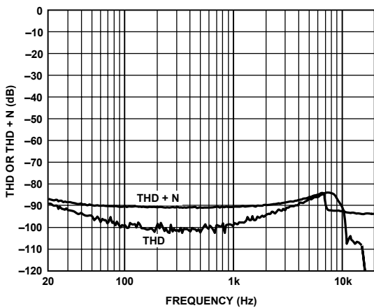
Figure 25. THD or THD + N vs. Frequency @ 1 W, 8 Ω, PVDD = 15 V, PGA = 0 dB
