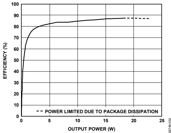
Figure 30. Efficiency vs. Output Power, 15 V, 6 Ω
