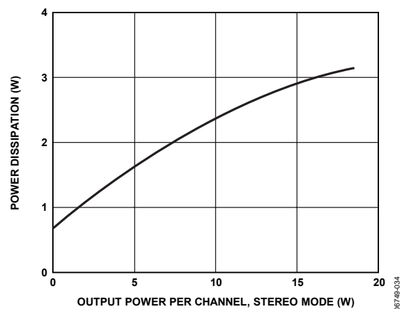
Figure 34. Power Dissipation vs. Output Power, 15 V, 8 Ω, Stereo Mode, Both Channels Driven
