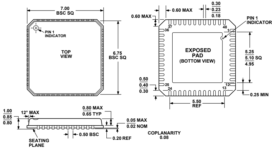
Figure 51. 48-Lead Lead Frame Chip Scale Package [LFCSP_VQ] 7 mm × 7 mm Body, Very Thin Quad (CP-48-1)
