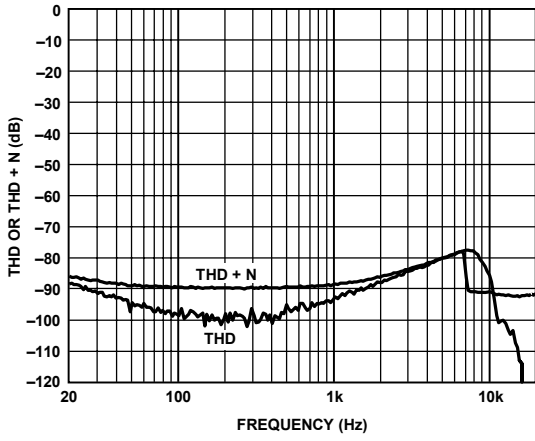
Figure 24. THD or THD + N vs. Frequency @ 1 W, 6 Ω, PVDD = 15 V, PGA = 0 dB
