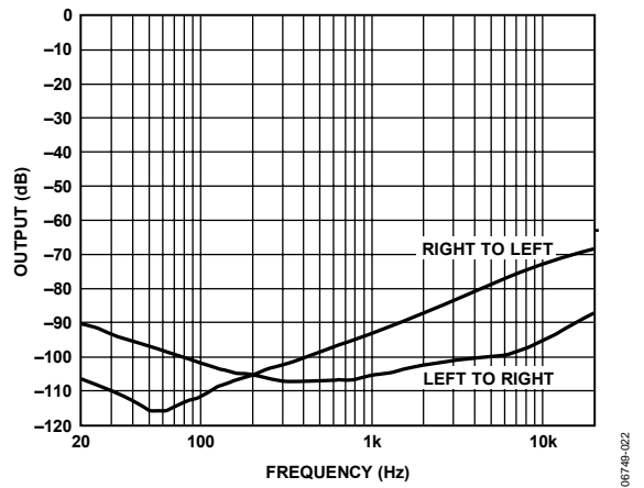
Figure 22. Crosstalk @ Full Scale, 6 Ω, PVDD = 15 V, PGA = 0 dB
