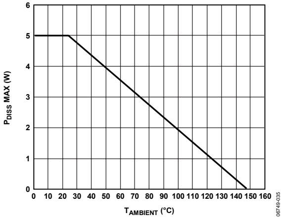
Figure 35. Power Dissipation Derating vs. Ambient Temperature
