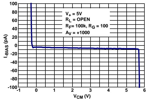
FIGURE 14. INPUT BIAS CURRENT vs COMMON-MODE INPUT VOLTAGE
