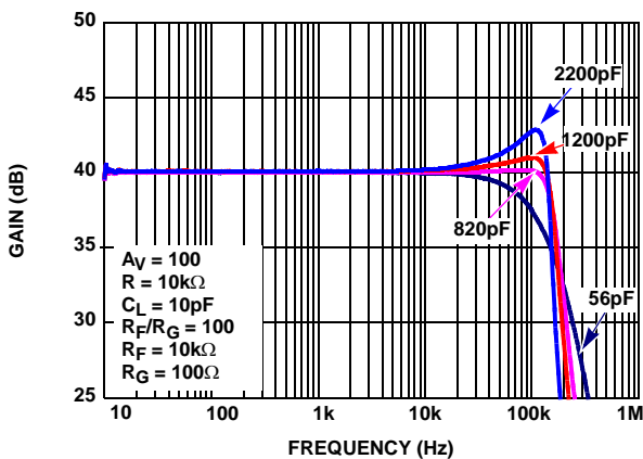
FIGURE 5. AMPLIFIER "A" (IN-AMP) FREQUENCY RESPONSE vs C_{LOAD}
