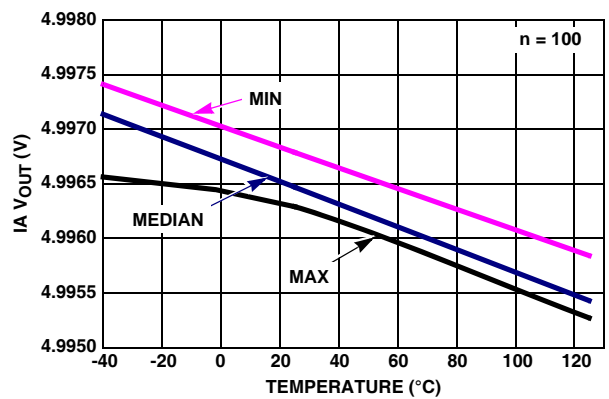
FIGURE 54. IA V_{OUT} HIGH vs TEMPERATURE, R_L = 100k, V_+, V_- = \pm 2.5V
