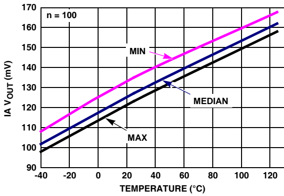
FIGURE 55. IA V_{OUT LOW} vs TEMPERATURE, R_L = 1k, V_+, V_- = \pm 2.5V
