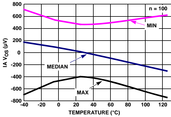
FIGURE 45. IA INPUT OFFSET VOLTAGE vs TEMPERATURE, V_+, V_- = \pm 2.5V
