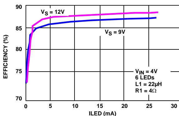
FIGURE 8. EFFICIENCY IMPROVEMENT WITH 9V AND 12V INPUTS
