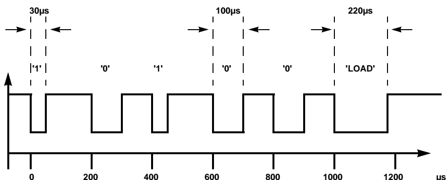
FIGURE 1. 1-WIRE XSD INTERFACE
