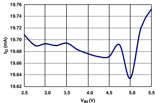
FIGURE 5. LINE REGULATION
