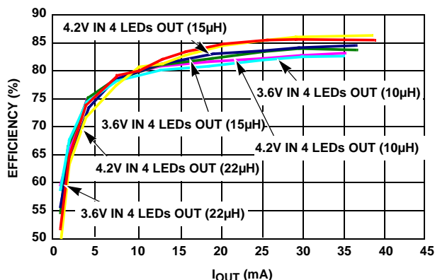
FIGURE 2. EFFICIENCY vs LED CURRENT
