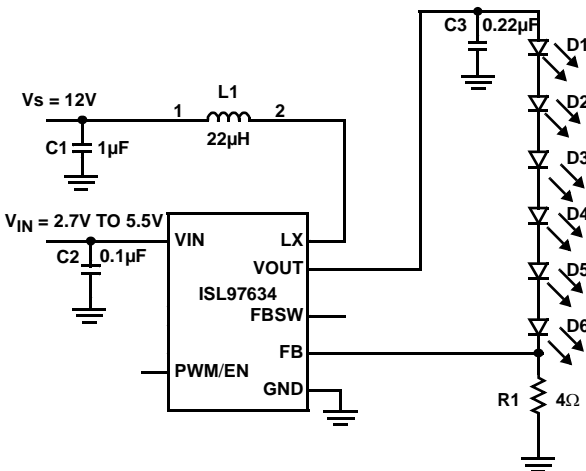
FIGURE 16. SEPARATE HIGH INPUT VOLTAGE FOR HIGHER EFFICIENCY OPERATION
