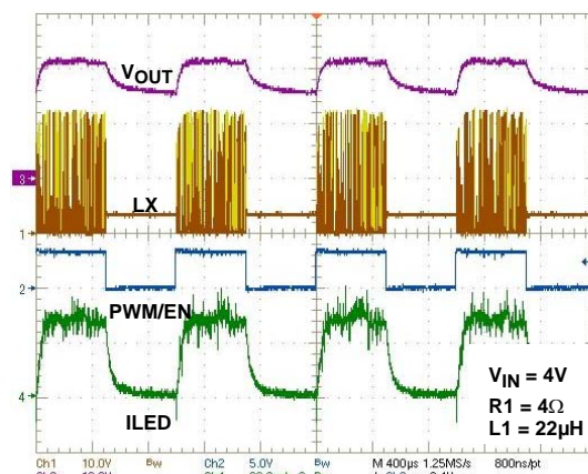
FIGURE 13. PWM DIMMING AT 1kHz WITHOUT USING FBSW
