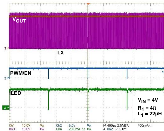
FIGURE 9. PWM DIMMING AT 1kHz, D = 99%
