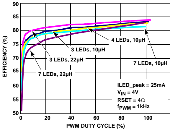
FIGURE 2. EFFICIENCY vs PWM DUTY CYCLE
