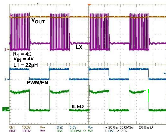
FIGURE 10. PWM DIMMING AT 20kHz, D = 50%
