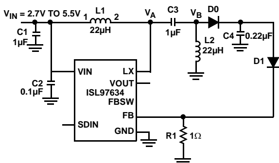
FIGURE 19. SEPIC LED DRIVER
