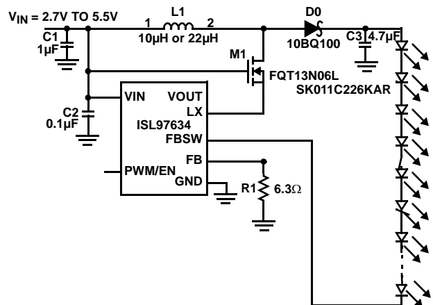
FIGURE 18. HIGH VOLTAGE LED DRIVER USING A CASCODE
