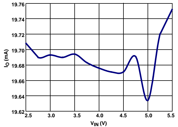
FIGURE 5. LINE REGULATION
