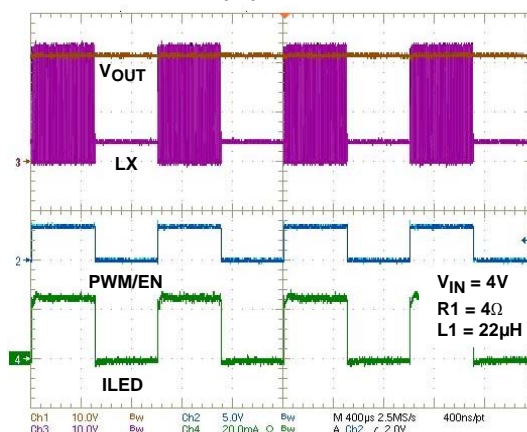
FIGURE 14. PWM DIMMING AT 1kHz USING FBSW
