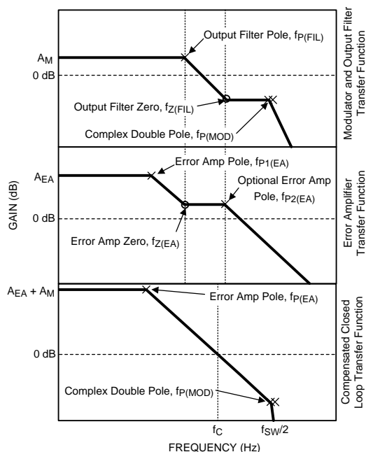
Figure 32. LM20133 Loop Compensation
