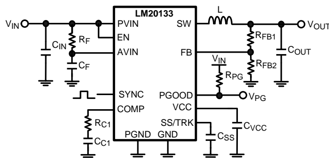
Figure 30. Typical Application Circuit
