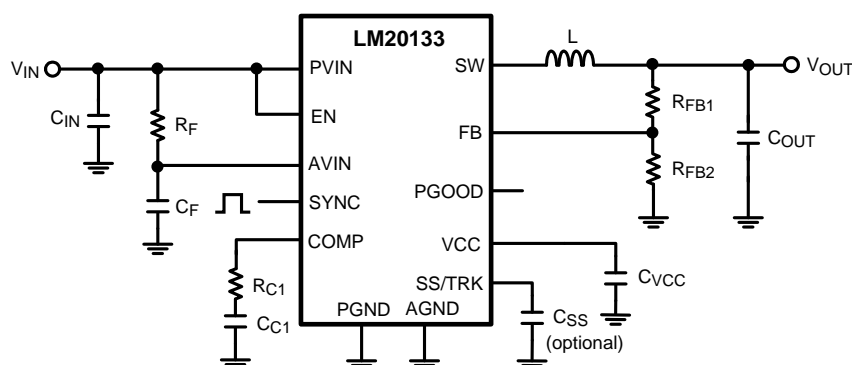
Typical Application Circuit
