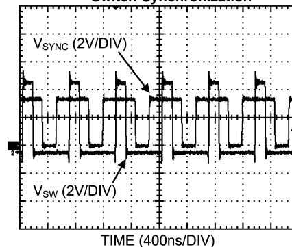
Switch Synchronization
