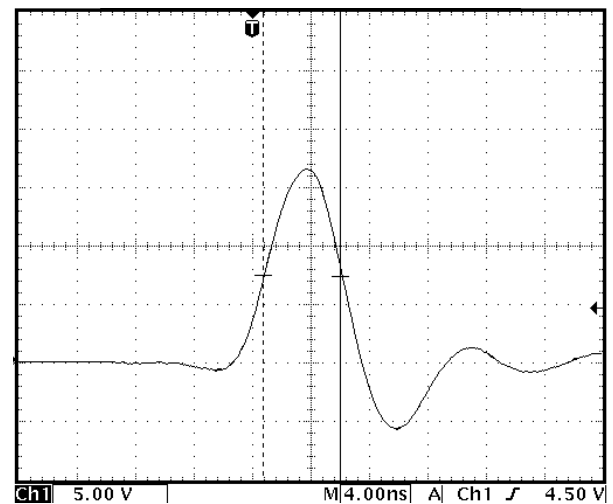
Figure 11 <6ns Minimum Pulse Width
