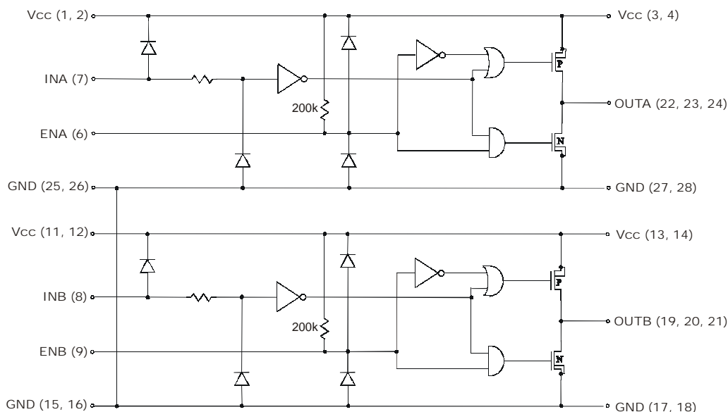
Figure 1 - Functional Diagram
