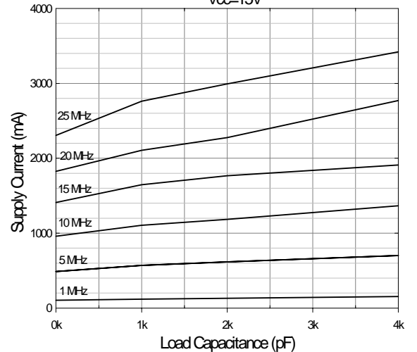
Fig. 6 Supply Current vs. Load Capacitance V CC = 15V
