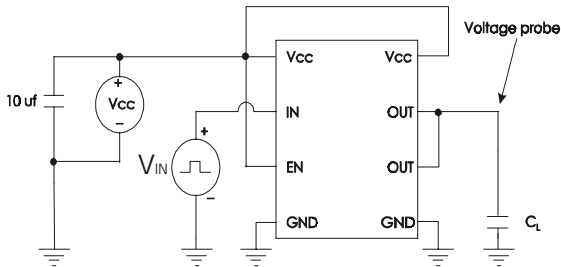
Figure 2a - Characteristics Test Diagram
