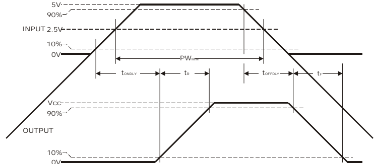
Figure 2b - Timing Diagram
