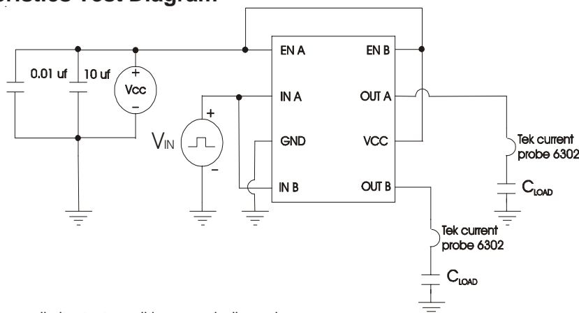
Figure 3 - Characteristics Test Diagram
