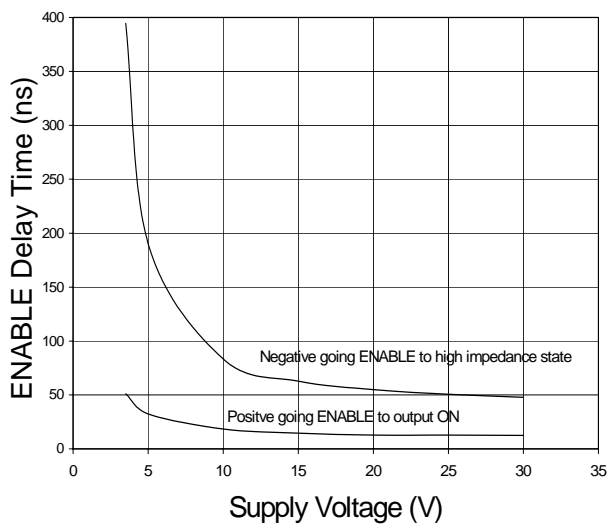
ENABLE Propagation Time vs. Supply Voltage
