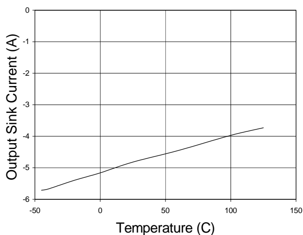
Fig. 25 Output Sink Current vs. Temperature V_{\text{SUPPLY}} = 15\text{V}
