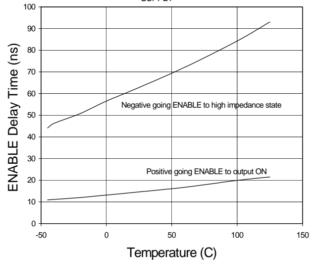
ENABLE Propagation Time vs. Temperature V_{\text{SUPPLY}} = 15\text{V}
