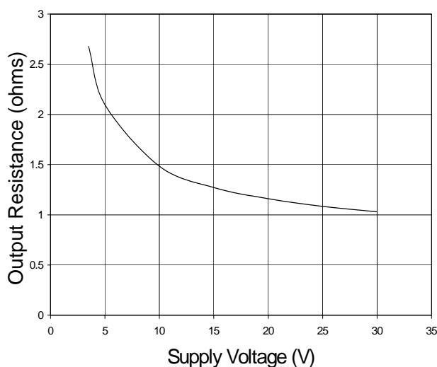
Fig. 27 Low State Output Resistance vs. Supply Voltage
