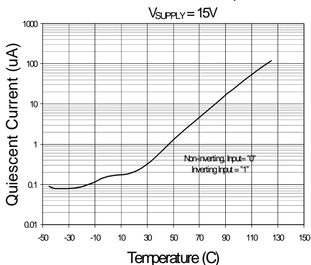
Fig. 15 Quiescent Current vs. Temperature
