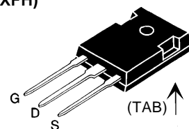
TO-268 (D3) (IXFT)
