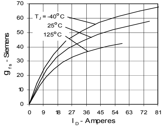
Fig. 8. Transconductance
