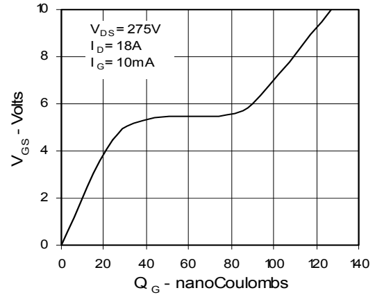
Fig. 10. Gate Charge
