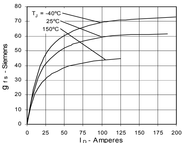
Fig. 8. Transconductance
