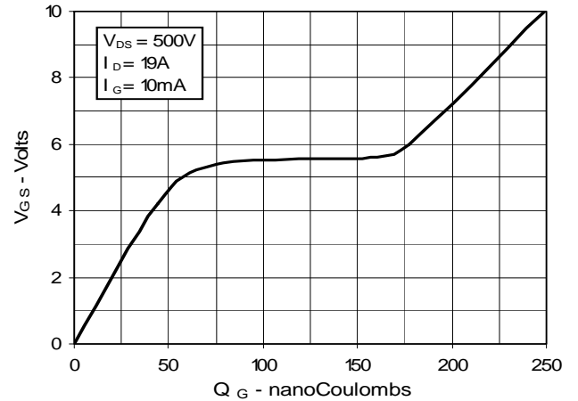
Fig. 10. Gate Charge
