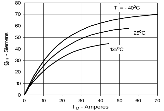
Fig. 8. Transconductance
