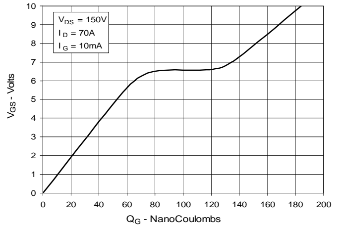
Fig. 10. Gate Charge
