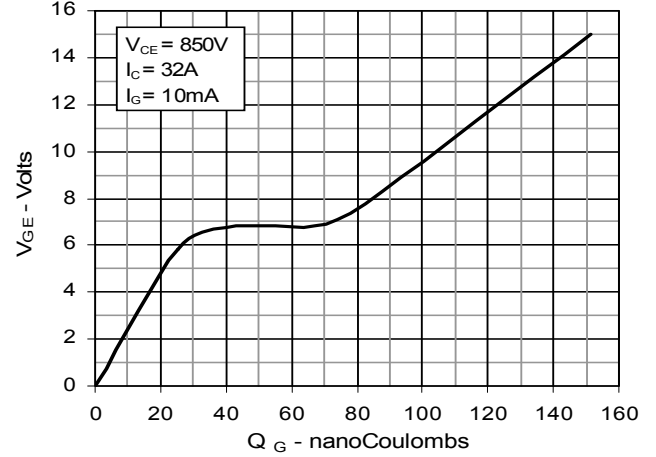
Fig. 8. Gate Charge
