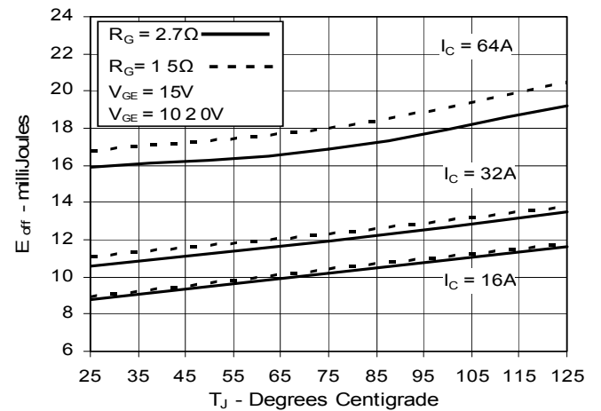
Fig. 12. Dependence of E_{off} on Temperature
