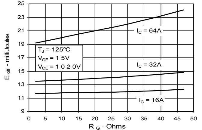
Fig. 10. Dependence of E_{off} on R_G
