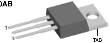
1 = Gate; 2, TAB = Collector; 3 = Emitter
