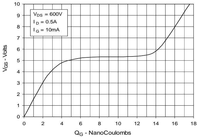
Fig. 9. Gate Charge
