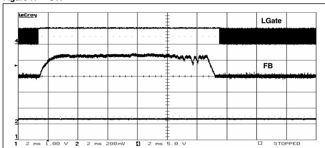
Figure 7. OVP
