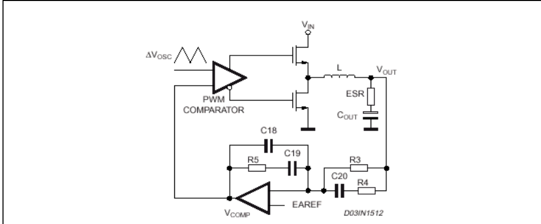
Figure 11. Compensation network
