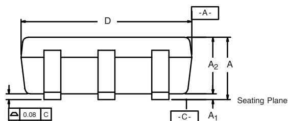
5-LEAD TSOP
