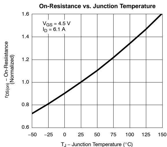
FIGURE 4. Si3434DV
