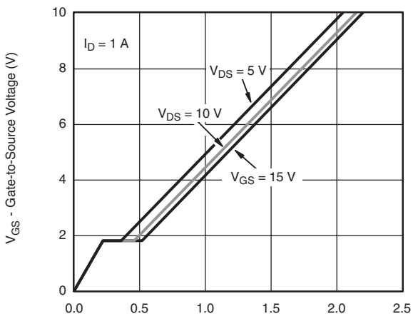
Gate Charge
