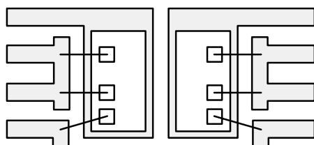
b) 8-Pin Dual-Pad TSSOP
