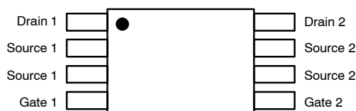
Figure 3. Pinouts for Dual-Die TSSOP
