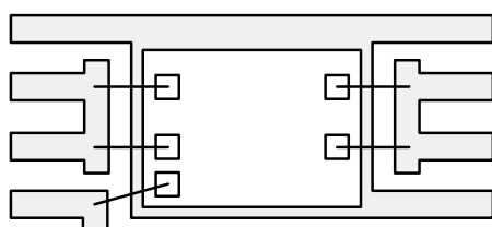
a) 8-Pin Single-Pad TSSOP
