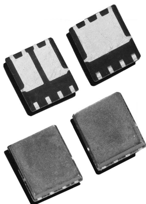
Figure 1. PowerPAK 1212 Devices
