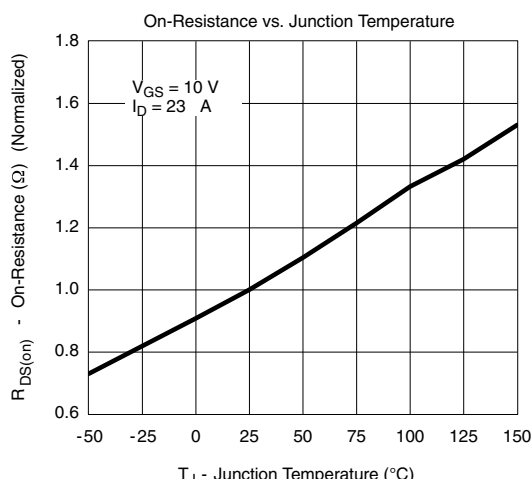
Fig. 7 MOSFET R_{DS(on)} vs. Temperature
