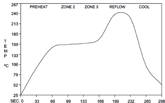
Fig. 3 Solder Reflow Temperature Profile
