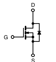
N-Channel MOSFET
