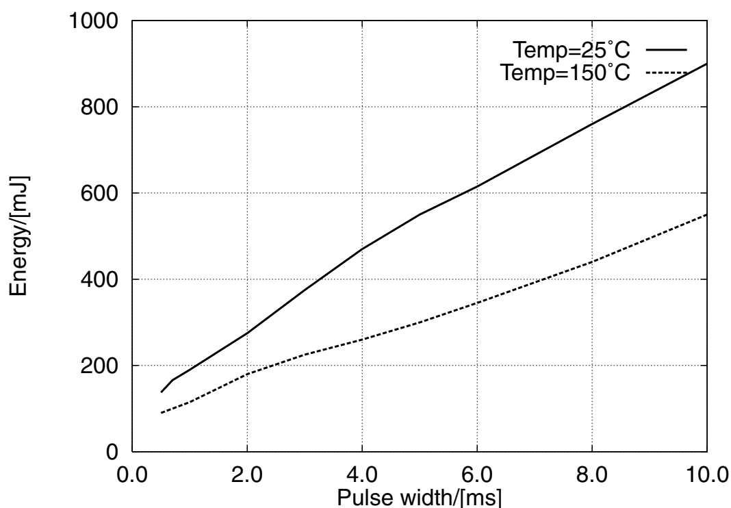
Figure 8. Max Clamp Energy Specification
