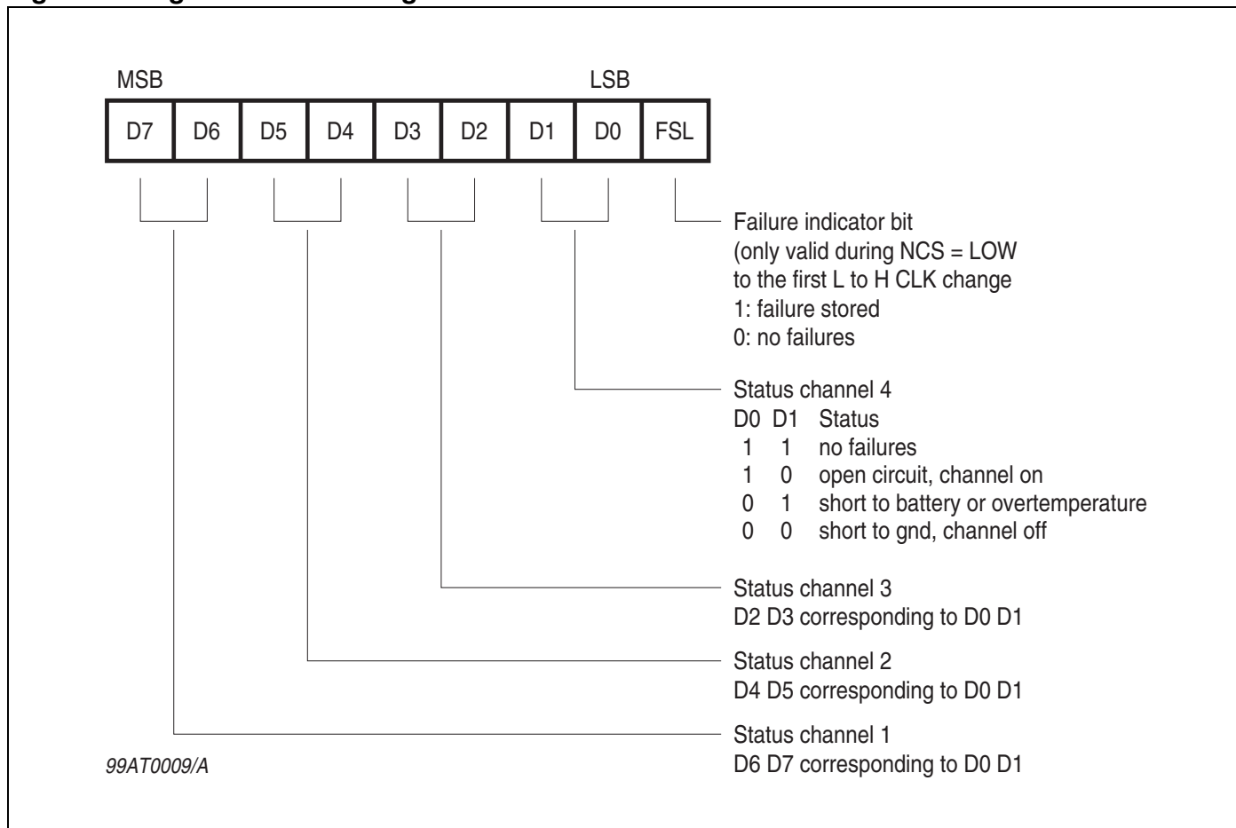
Figure 2. Diagnostic Failure Register Structure
