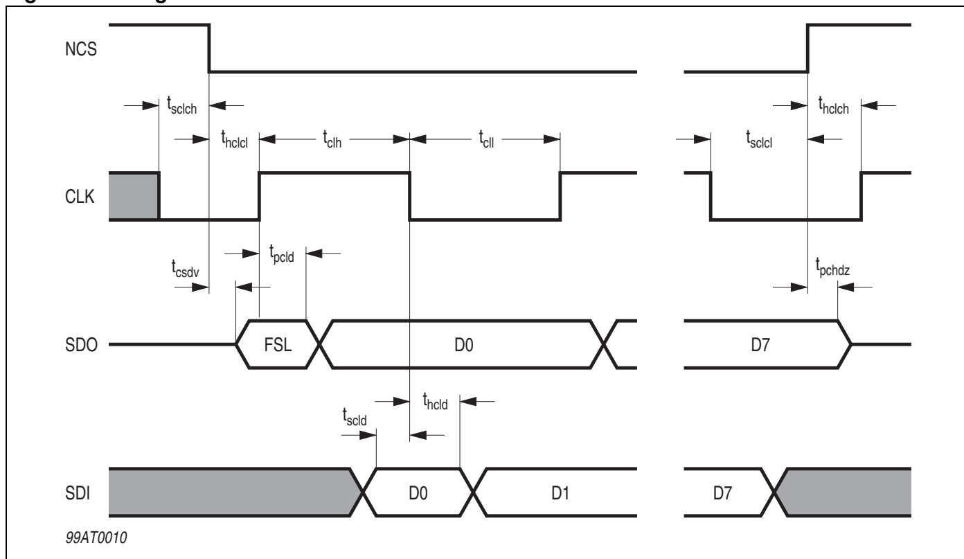
Figure 3. Timing of the Serial Interface
