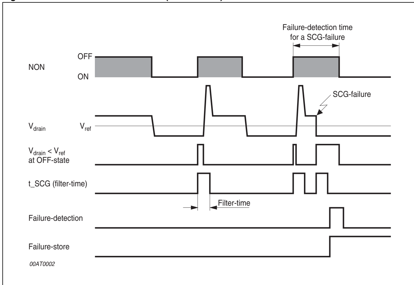
Figure 4. Short-Circuit to GND Failure (SCG-Failure) Detection
