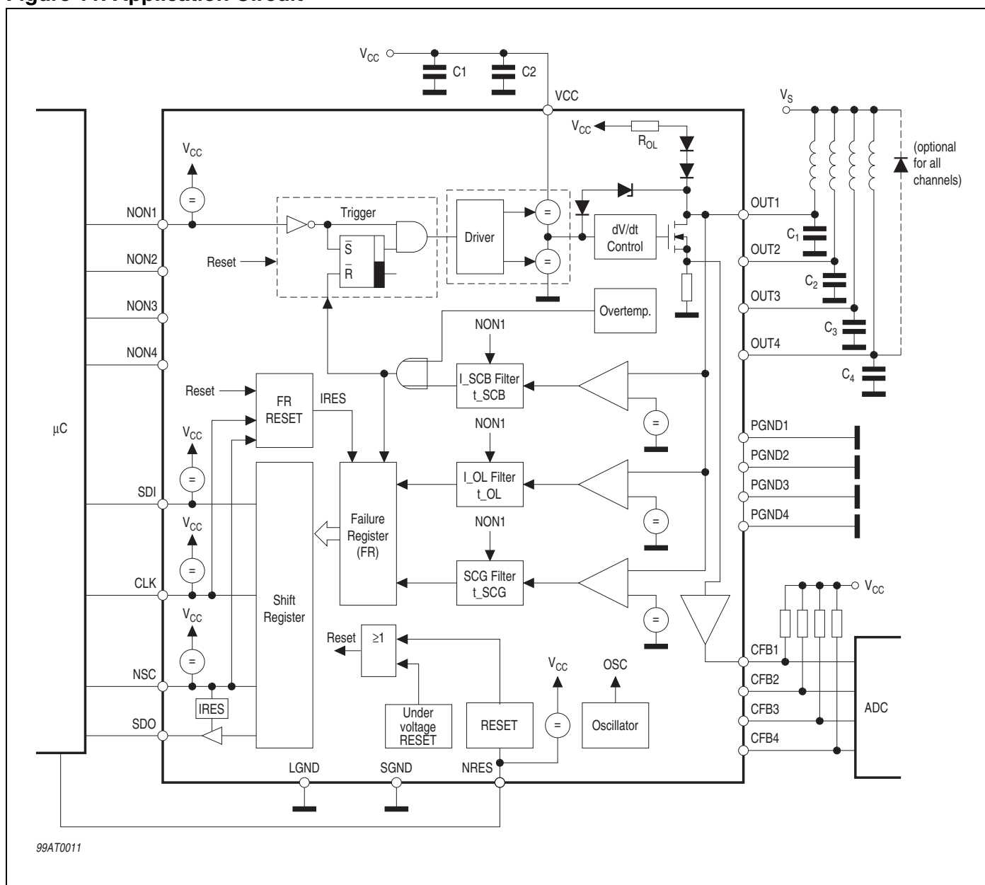
Figure 11. Application Circuit
