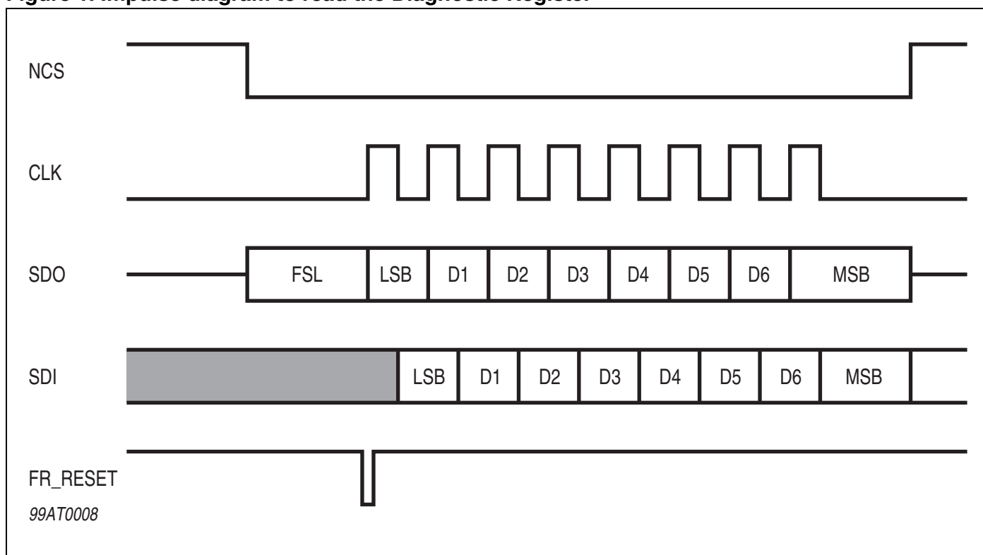
Figure 1. Impulse diagram to read the Diagnostic Register
