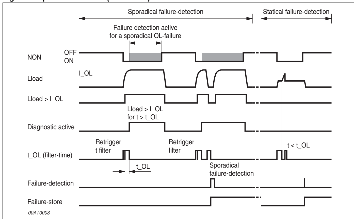
Figure 5. Open-Load Failure (OL-Failure) Detection
