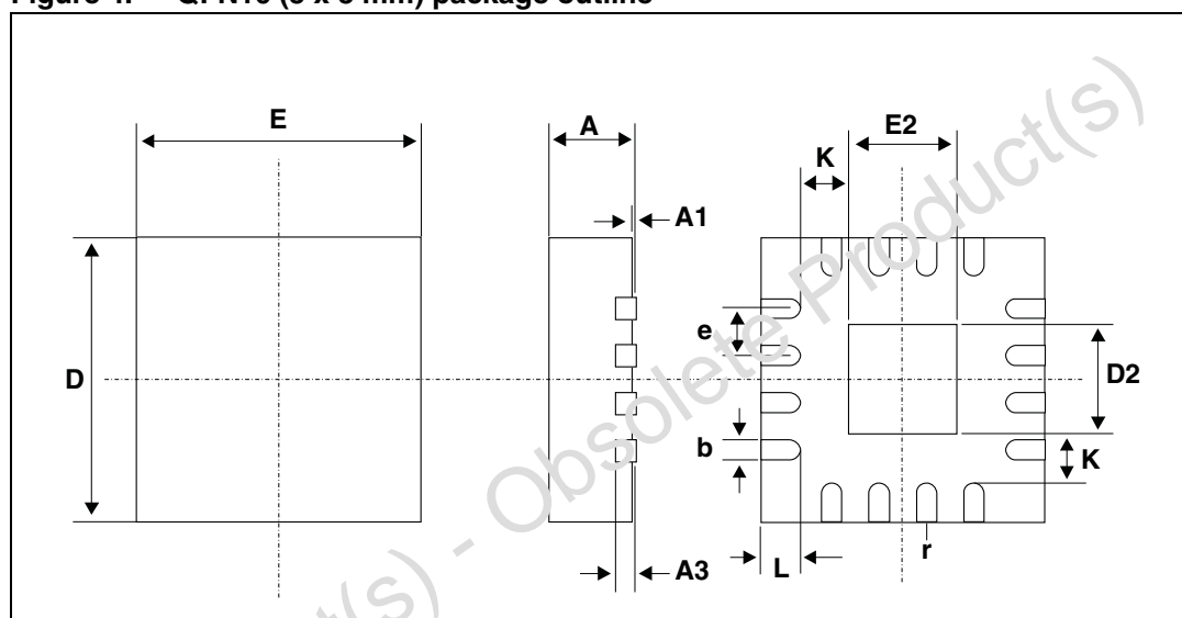
Figure 4. QFN16 (3 x 3 mm) package outline
