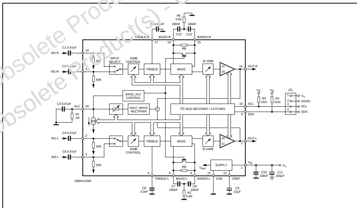
Figure 2. Application & Test Circuit
