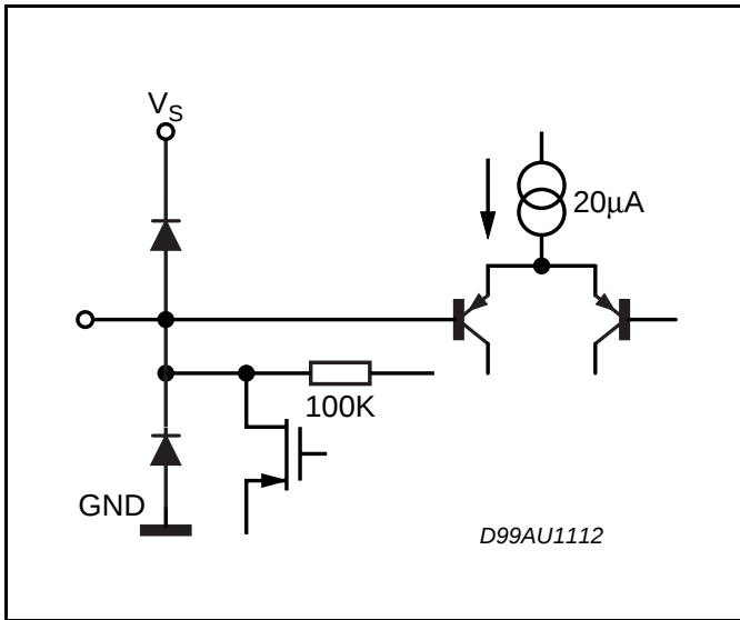
Figure 11. PIN CREF
