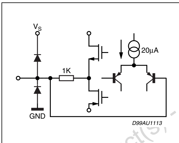
Figure 15. PIN: CREF
