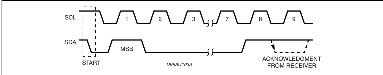
Figure 6. Acknowledge on the I 2 CBUS
