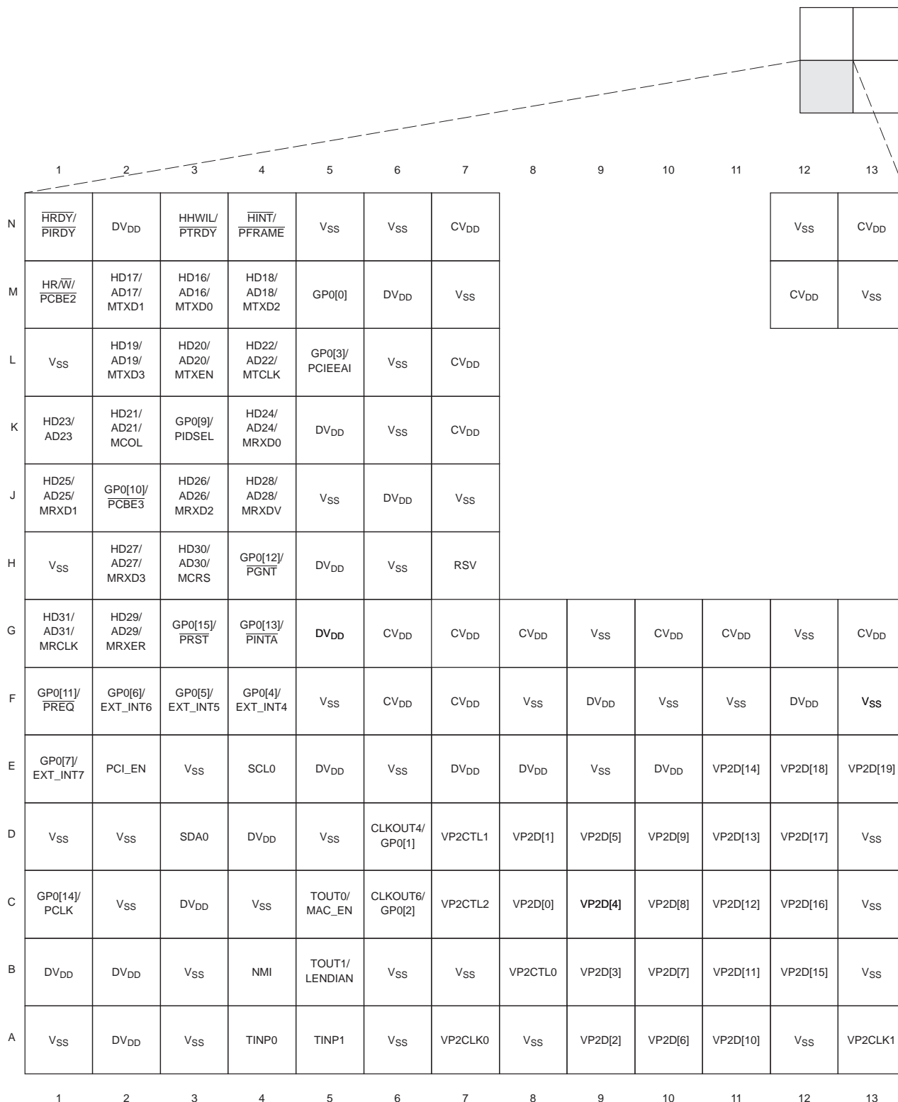
Figure 2-5. DM642 Pin Map [Quadrant C]
