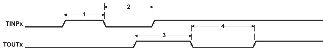
Figure 5-69. Timer Timing
