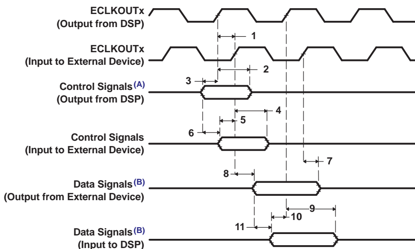
Figure 5-4. Board-Level Input/Output Timings
