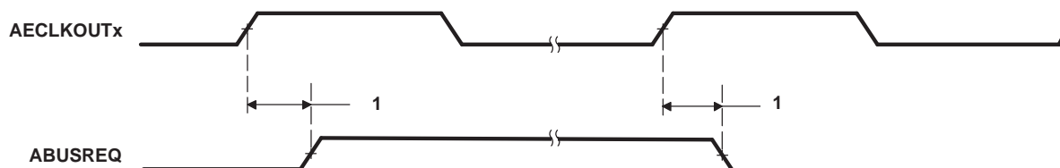
Figure 5-31. BUSREQ Timing for EMIFA
