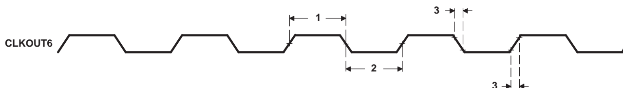
Figure 5-13. CLKOUT6 Timing
