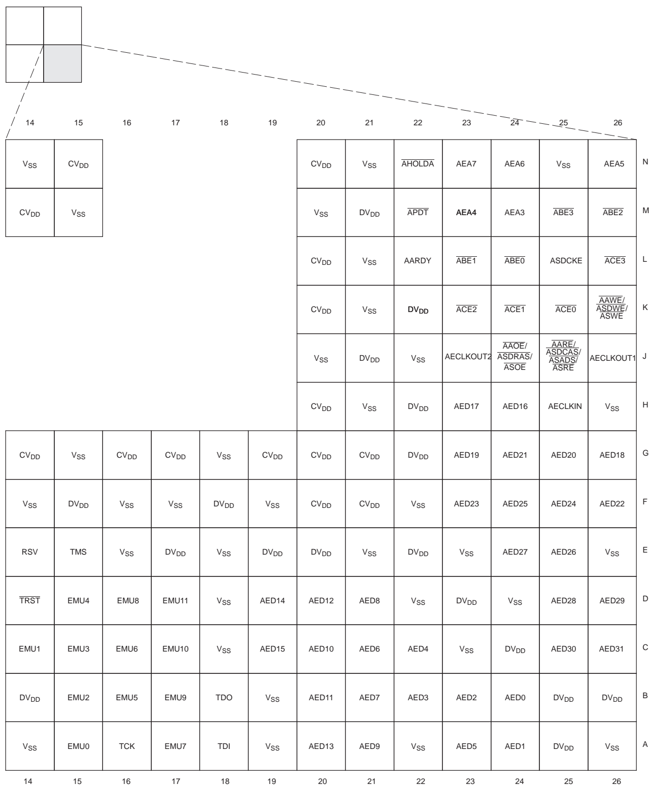
Figure 2-6. DM642 Pin Map [Quadrant D]
