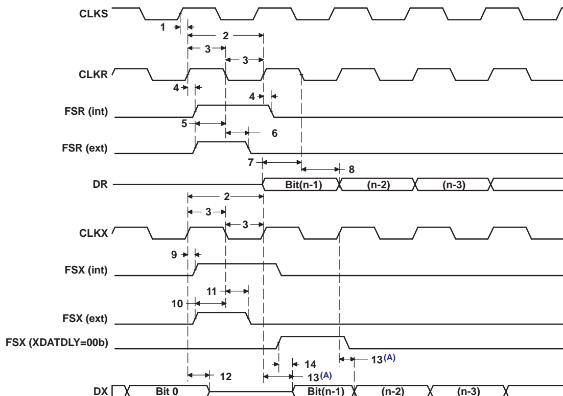
Figure 5-51. McBSP Timing
