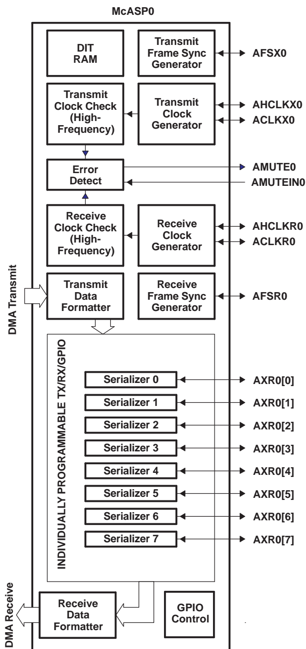
Figure 5-32. McASP0 Configuration
