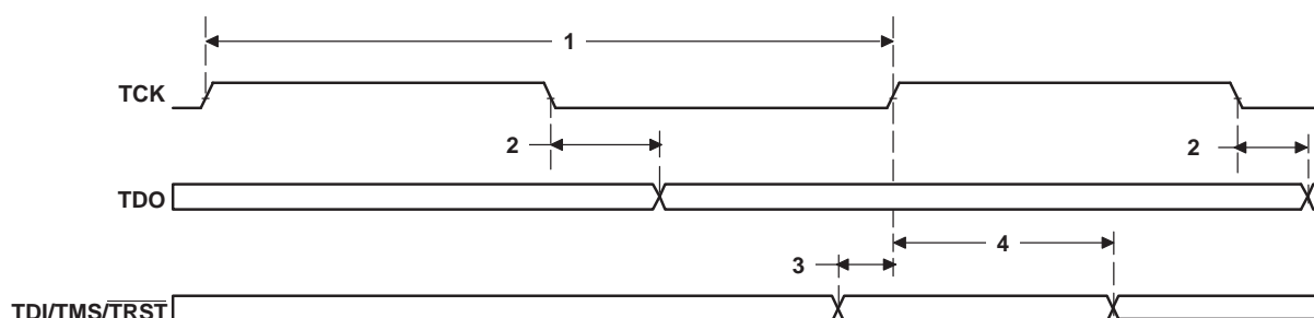
Figure 5-74. JTAG Test-Port Timing
