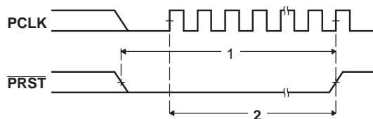
Figure 5-47. PCI Reset ( \overline{PRST} ) Timing
