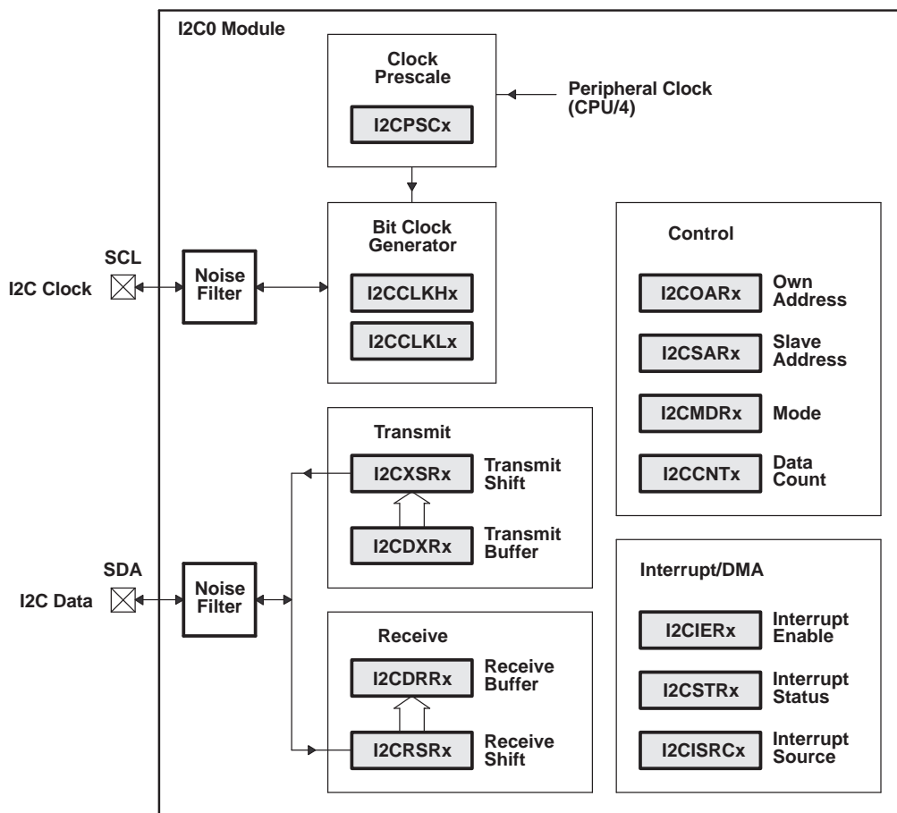
Figure 5-35. I2C0 Module Block Diagram
