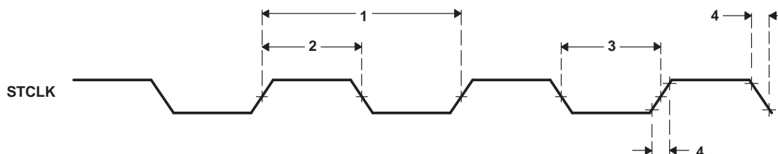
Figure 5-62. STCLK Timing
