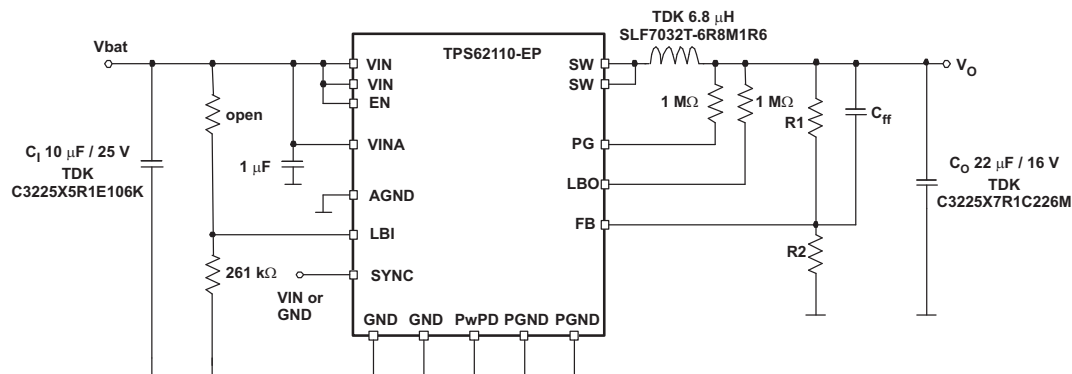
Figure 17. Test Setup
