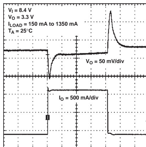
TPS62111 LOAD TRANSIENT
