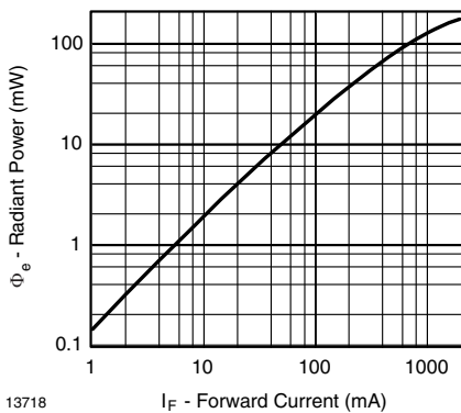
Fig. 4 - Radiant Power vs. Forward Current
