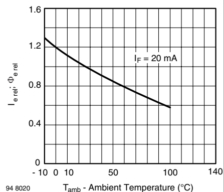
Fig. 8 - Rel. Radiant Intensity/Power vs. Ambient Temperature
