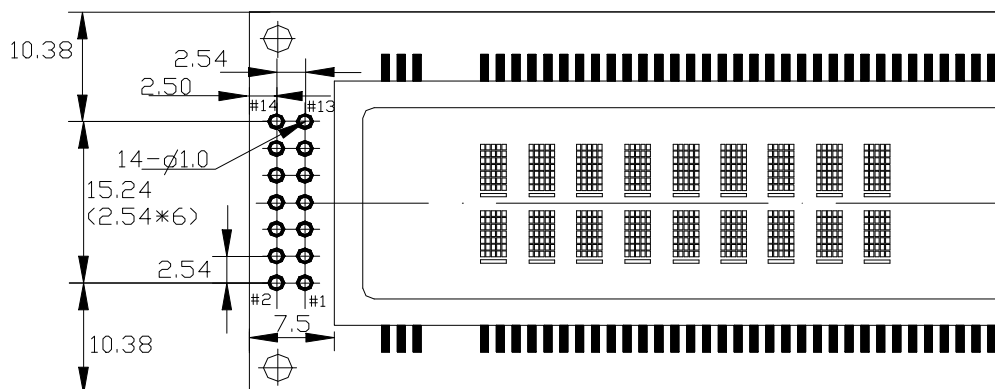
Fig-8 14-pin Through Hole Dimensions
