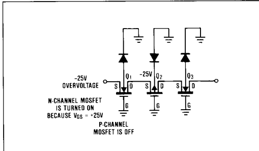
Figure 8. -25V Overvoltage with Multiplexer Power OFF
