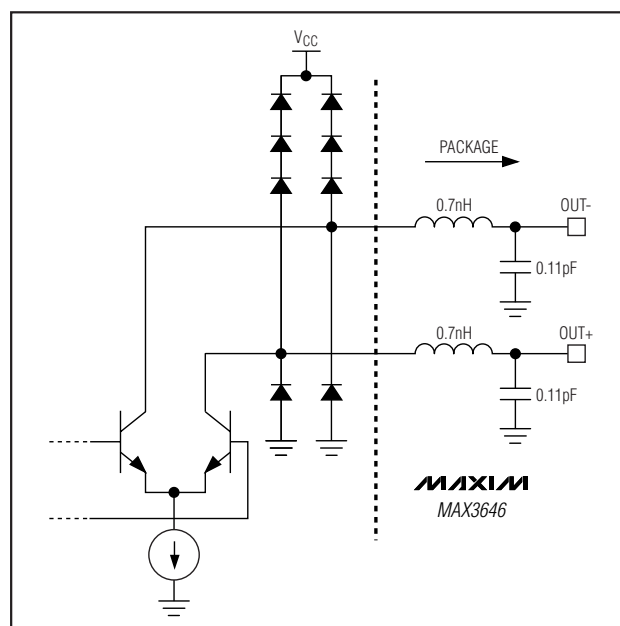
Figure 7. Simplified Output Structure
