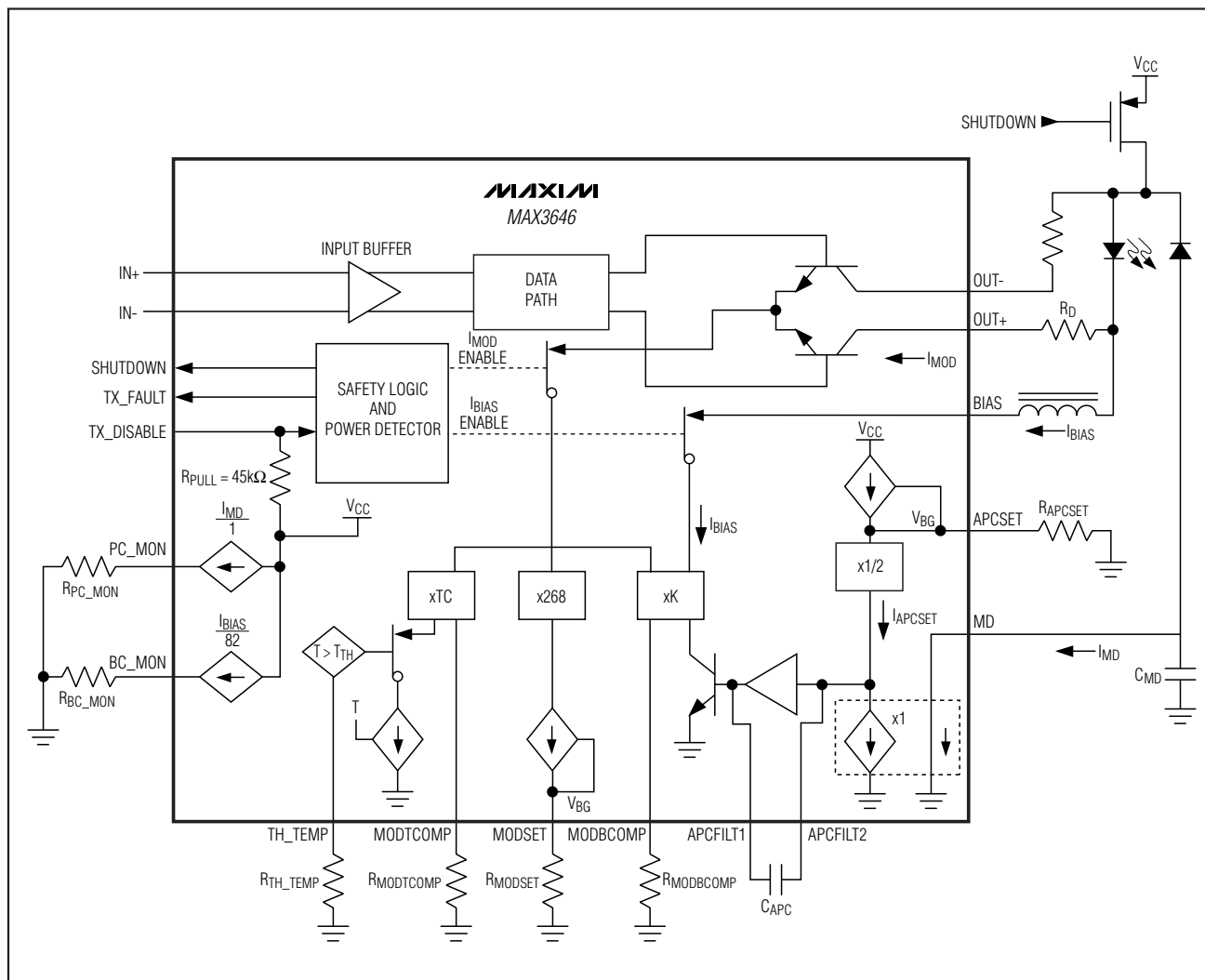
Figure 4. Functional Diagram
