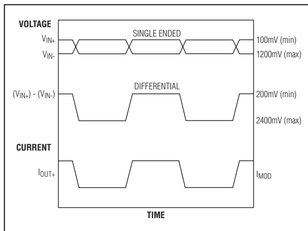
Figure 1. Required Input Signal and Output Polarity
