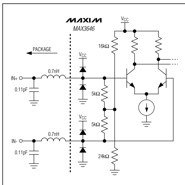
Figure 6. Simplified Input Structure
