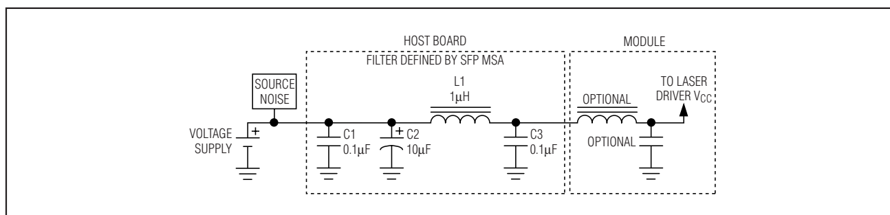
Figure 3. Supply Filter
