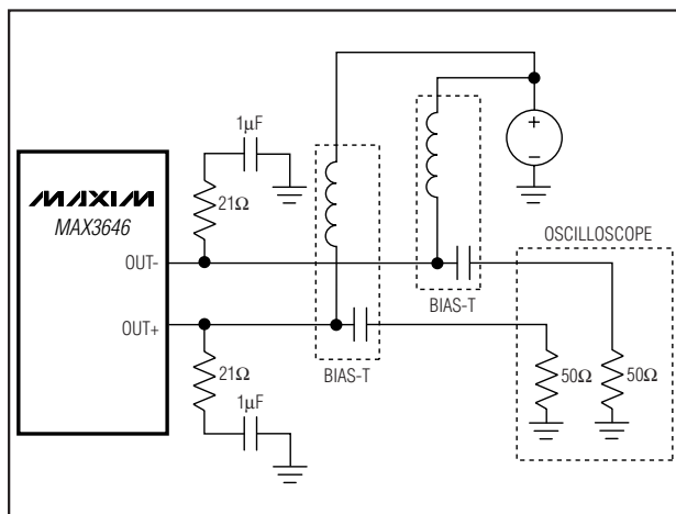
Figure 2. Test Circuit for Characterization
