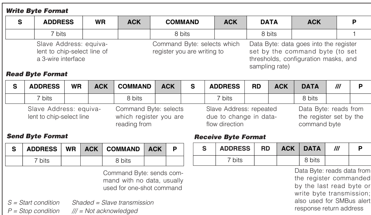
Figure 2. SMBus Protocols
