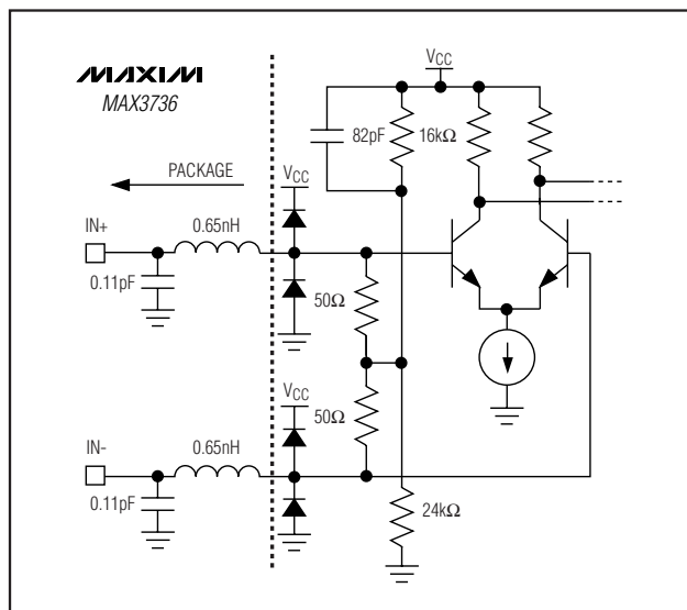
Figure 5. Simplified Input Circuit Schematic
