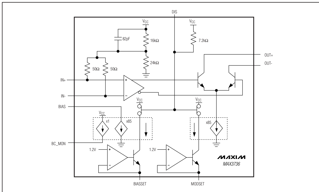
Figure 4. Functional Diagram
