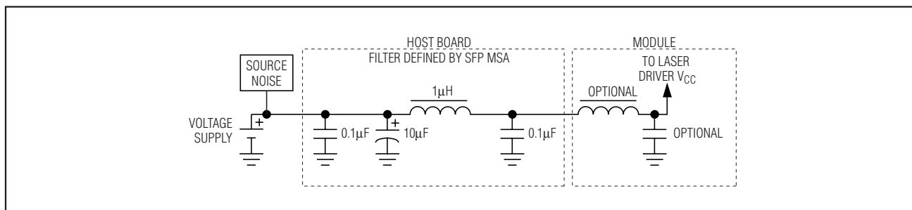
Figure 3. Supply Filter
