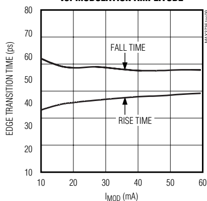
EDGE TRANSITION TIME vs. MODULATION AMPLITUDE
