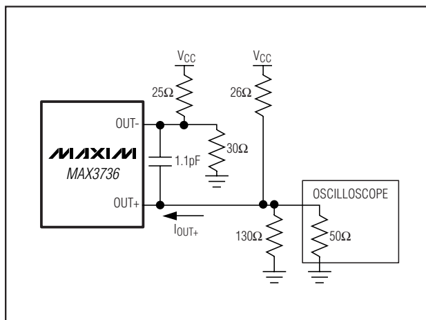
Figure 2. Output Termination for Characterization
