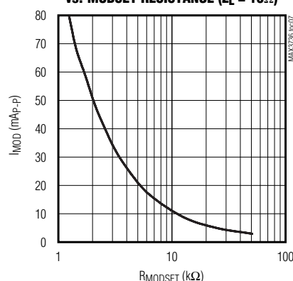
MODULATION CURRENT vs. MODSET RESISTANCE ( Z_L = 15\Omega )
