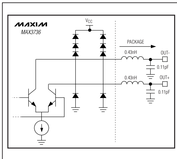
Figure 6. Simplified Output Circuit Schematic
