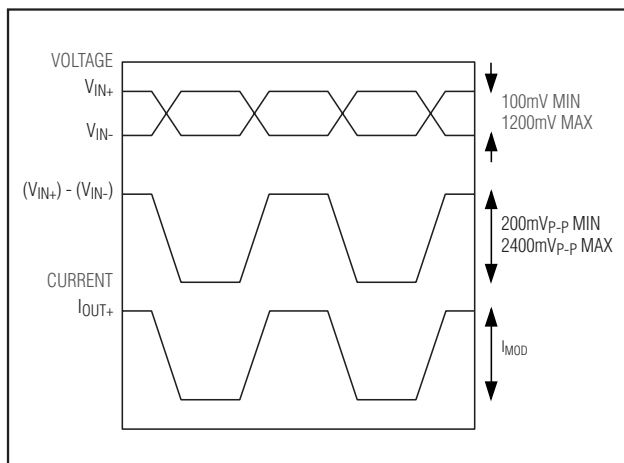
Figure 1. Definition of Single-Ended Input Voltage Range
