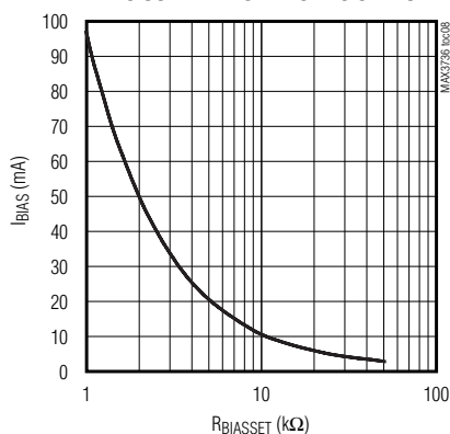
BIAS CURRENT vs. BIAS RESISTANCE
