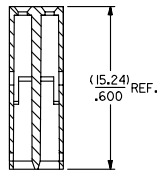
SECTION C-C
