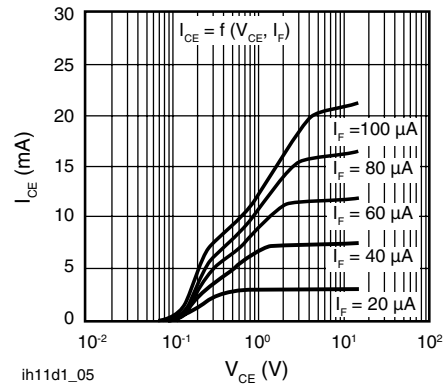
Fig. 4 - Output Characteristics
