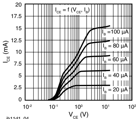
Fig. 3 - Output Characteristics
