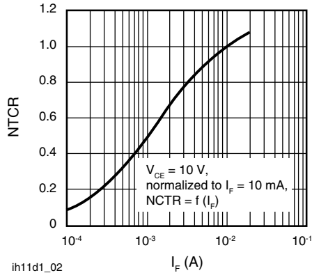
Fig. 1 - Current Transfer Ratio (typ.)
