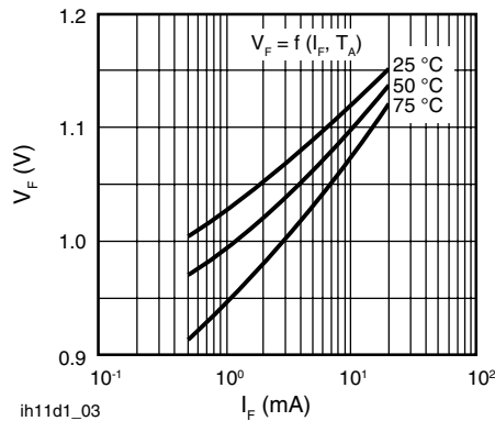
Fig. 2 - Diode Forward Voltage (typ.)
