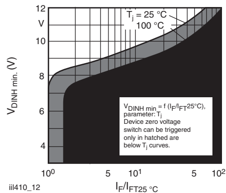
Fig. 10 - Typical Static Inhibit Voltage Limit
