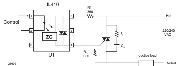
Fig. 16 - Basic Power Triac Driver Circuit
