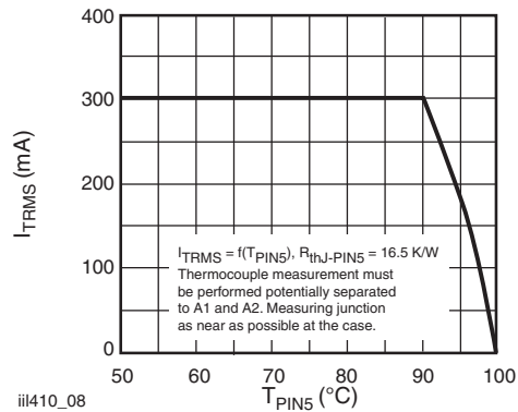
Fig. 6 - Current Reduction
