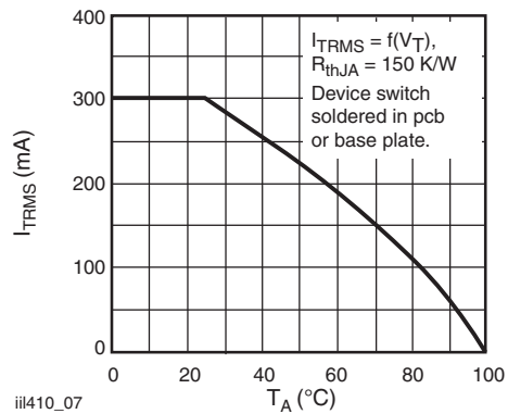
Fig. 5 - Current Reduction
