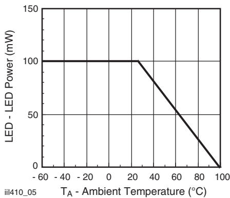
Fig. 3 - Maximum LED Power Dissipation
