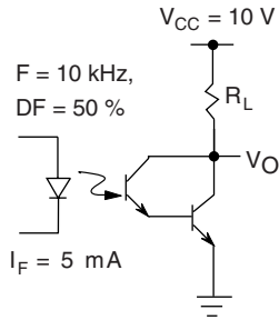
Fig. 8 - Switching Schematic
