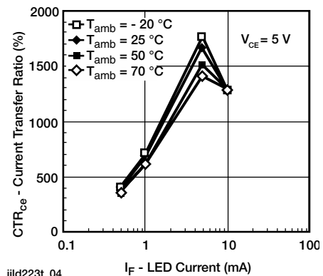
Fig. 6 - CTR vs. LED Current
