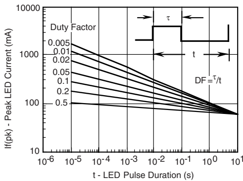
Fig. 4 - Peak LED Current vs. Duty Factor, \tau
