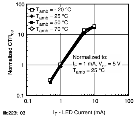
Fig. 5 - Normalized CTR CE vs. LED Current
