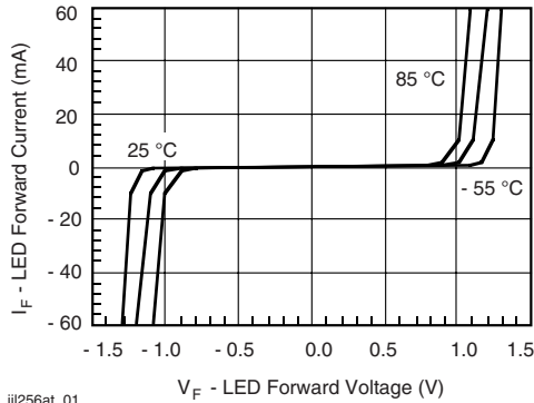
iii256at_01 Figure 1. LED Forward Current vs. Forward Voltage
