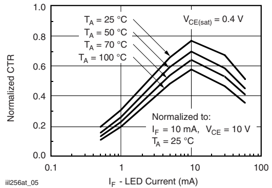
iii256at_05 Figure 5. Normalized Saturated CTR
