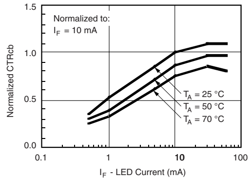
iii256at_06 Figure 6. Normalized CTR_{cb}
