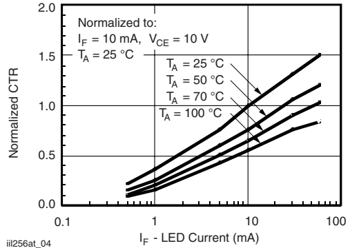
iii256at_04 Figure 4. Normalized CTR vs. I_F and T_{amb}
