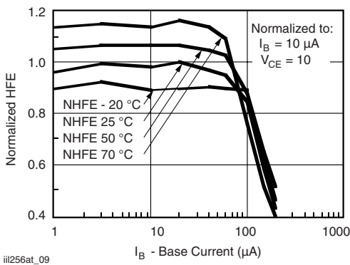
Figure 9. Normalized HFE vs. Base Current and Temp.
