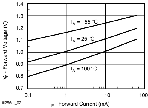
iii256at_02 Figure 2. Forward Voltage vs. Forward Current
