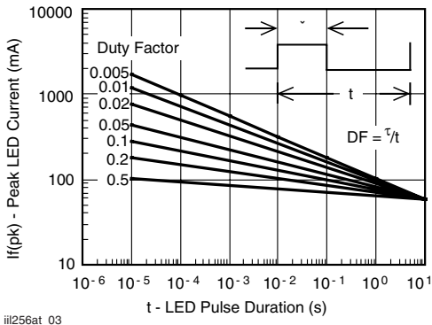
iii256at_03 Figure 3. Peak LED Current vs. Duty Factor, Tau
