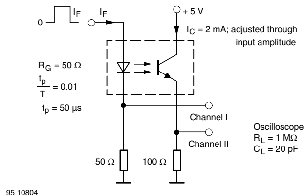
Fig. 1 - Test Circuit, Non-Saturated Operation
