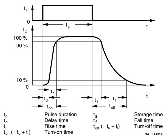
Fig. 3 - Switching Times
