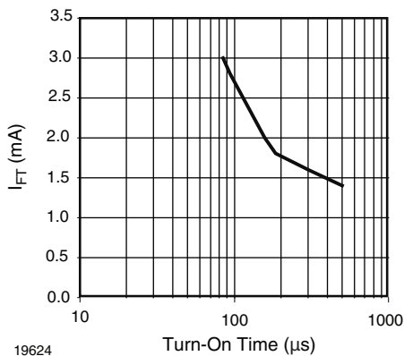
Fig. 8 - Trigger Current vs. Turn-On Time
