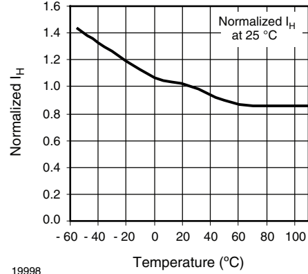
Fig. 9 - Normalized Holding Current vs. Temperature
