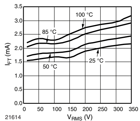
Fig. 11 - I_{FT} vs. V_{RMS} and Temperature
