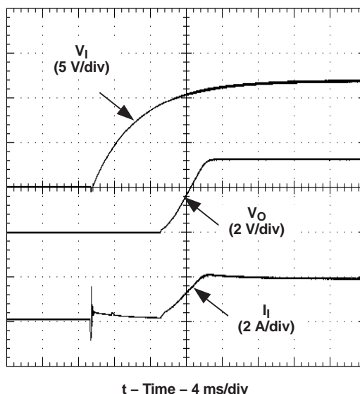
Figure 13. Power-Up Waveforms
