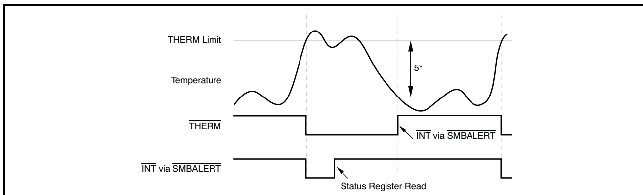
Figure 23. Operation of the THERM Interrupt and the THERM Pin
