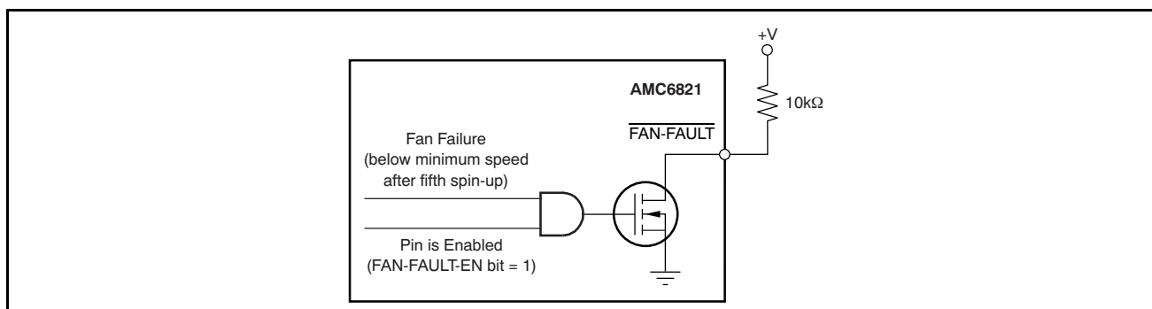
Figure 21. \overline{\text{FAN-FAULT}} Pin
