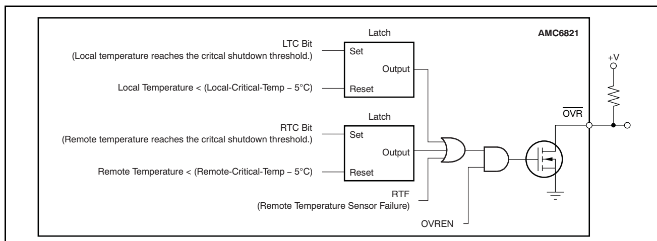
Figure 30. \overline{\text{OVR}} Pin
