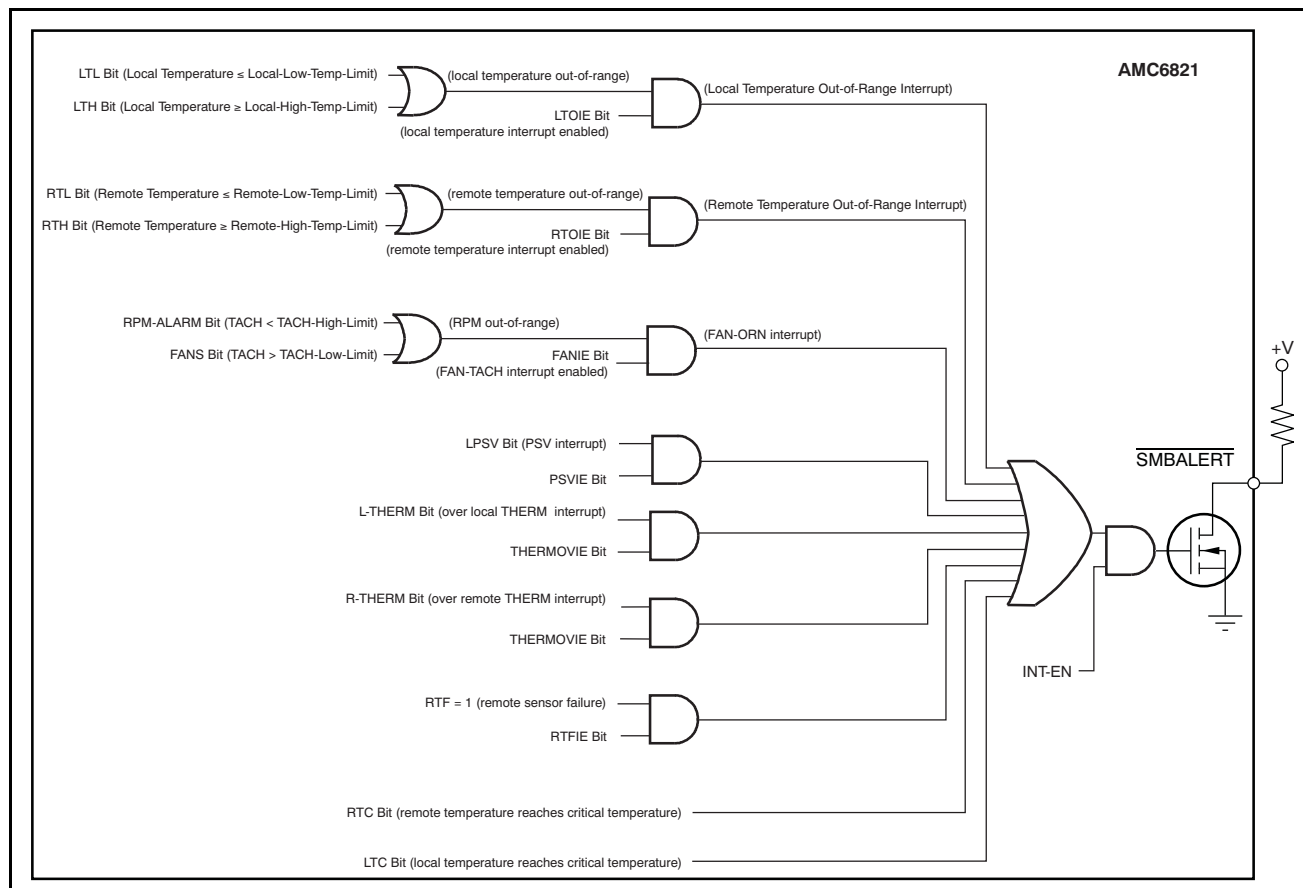
Figure 33. SMBALERT
