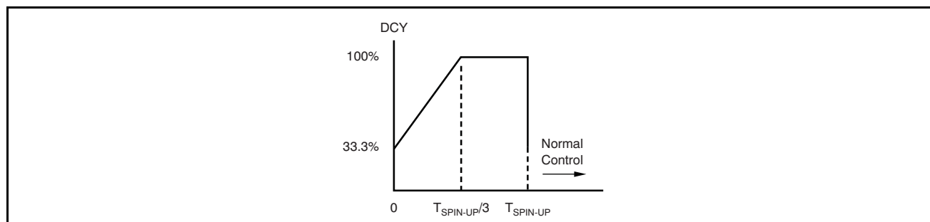
Figure 24. Spin-Up Process
