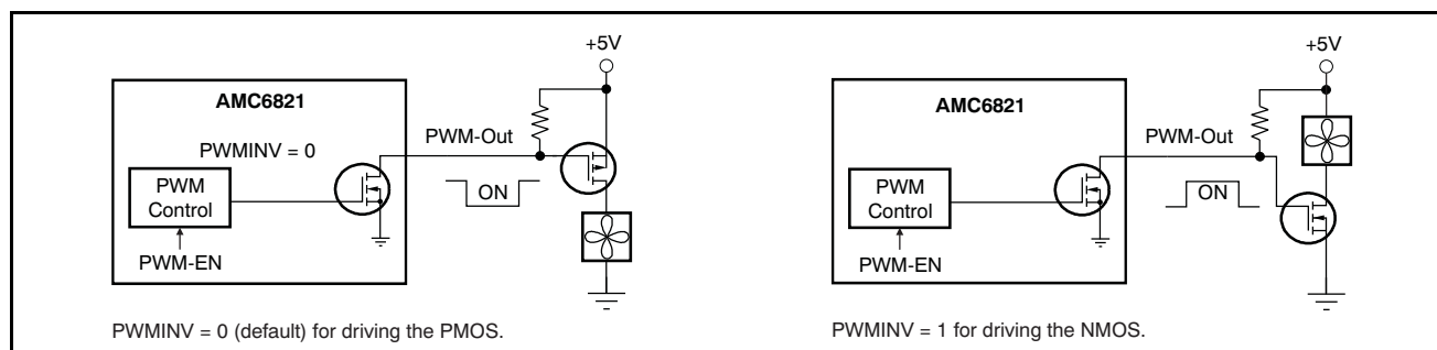
Figure 15. PWM Output
