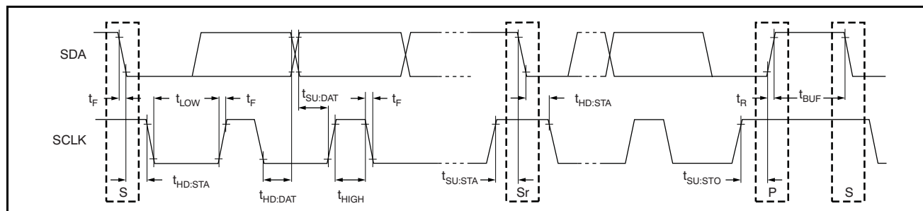
Figure 1. Timing Specification
