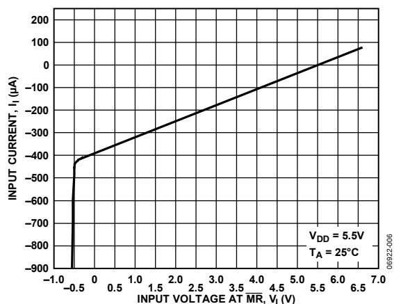
Figure 6. Input Current vs. Input Voltage at \overline{\text{MR}}
