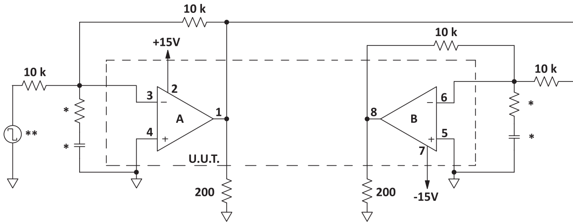
Figure 1: Burn in Circuit
