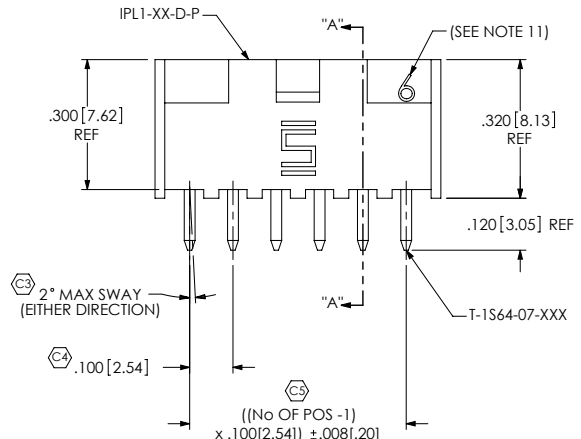
FIG 1 IPL1-106-01-XXX-D-P SHOWN
