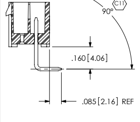
FIG 5 (IPL1-106-01-XXX-D-K SHOWN) (DIFFERENT AS SHOWN, OTHERWISE SAME AS FIG 4)
