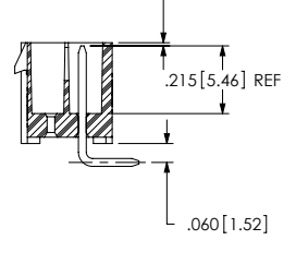
FIG 6 (IPL1-106-01-XXX-D-RA-G SHOWN) (DIFFERENT AS SHOWN, OTHERWISE SAME AS FIG 3)
