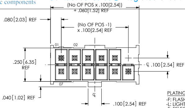
FIG 1 IPL1-106-01-XXX-D-P SHOWN
