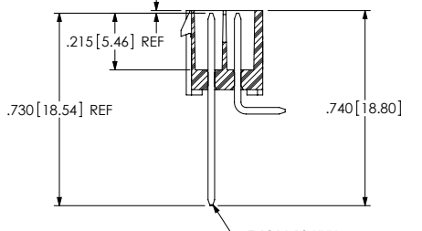
FIG 7 (IPL1-102-01-XXX-D-G SHOWN) (DIFFERENT AS SHOWN, OTHERWISE SAME AS FIG 1)
