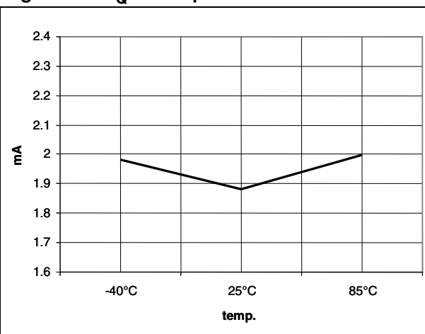
Figure 20. I_Q vs temp
