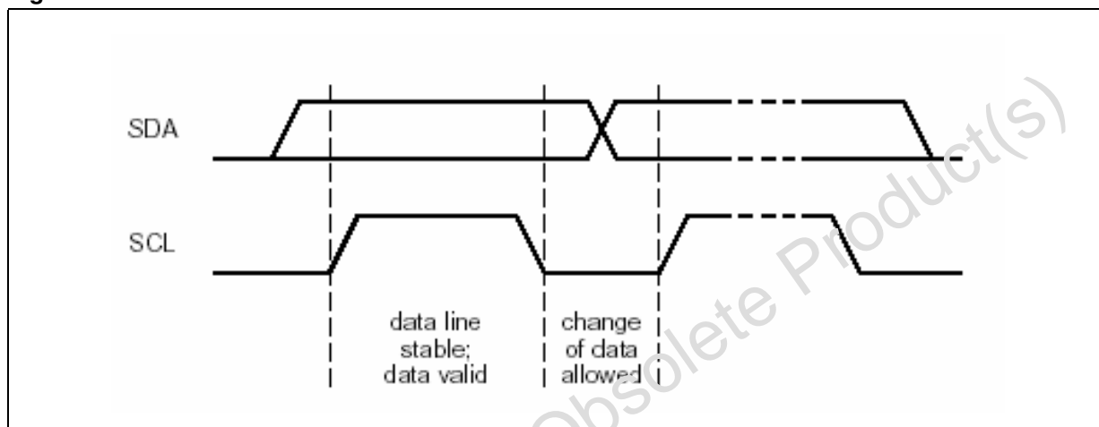
Figure 7. Bit transfer
